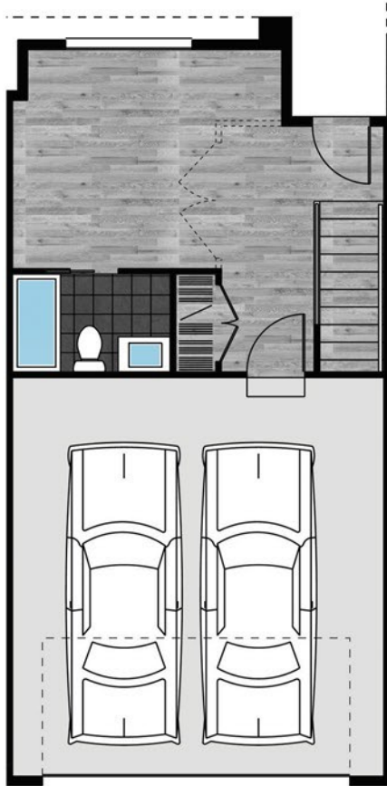
1ST FLOOR
